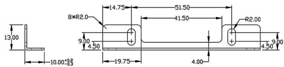
bracket part# 360220037-00
