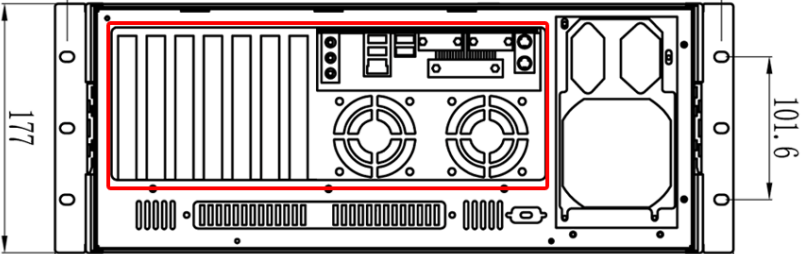
chassis with standard ATX 7 slot rear panel(R4450A-7S-RP)
